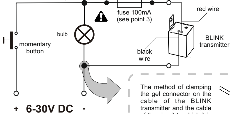
Fig. 3 An exemplary electrical diagram of connecting the BLINK transmitter to the bulb circuit.
